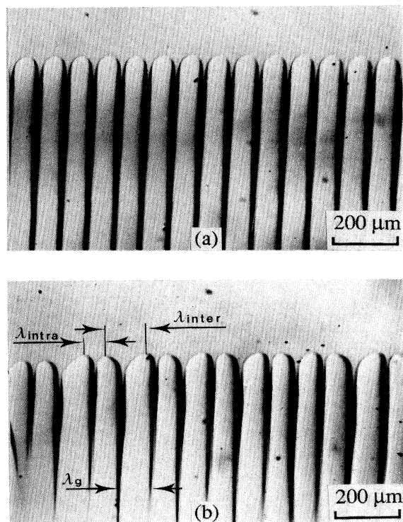
FIG. 1. (a) Regular cellular array. Succinonitrile–0.15 wt. % acetone. V=5 \mu\text{m/s} . G=62^\circ\text{C/cm} . \nu=2.4 . (b) Doublet interface. Succinonitrile–0.15 wt. % acetone. V=4 \mu\text{m/s} . G=65^\circ\text{C/cm} . \nu=1.8 .
