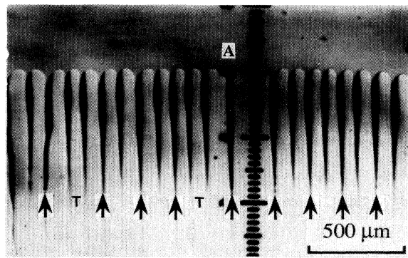
FIG. 13. Coexistence of doublets with triplets (the arrows indicate the intergrooves). Succinonitrile-0.15 wt. % acetone. V = 4 \mu\text{m/s} . G = 65^\circ\text{C/cm} . \nu = 1.8 .
