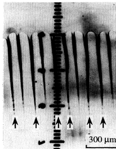
FIG. 14. Two individual cells in an array of doublets, with meandering of the intergrooves (arrows). Succinonitrile-0.15 wt. % acetone. V = 4 \mu\text{m/s} . G = 59^\circ\text{C/cm} . \nu = 2 .
